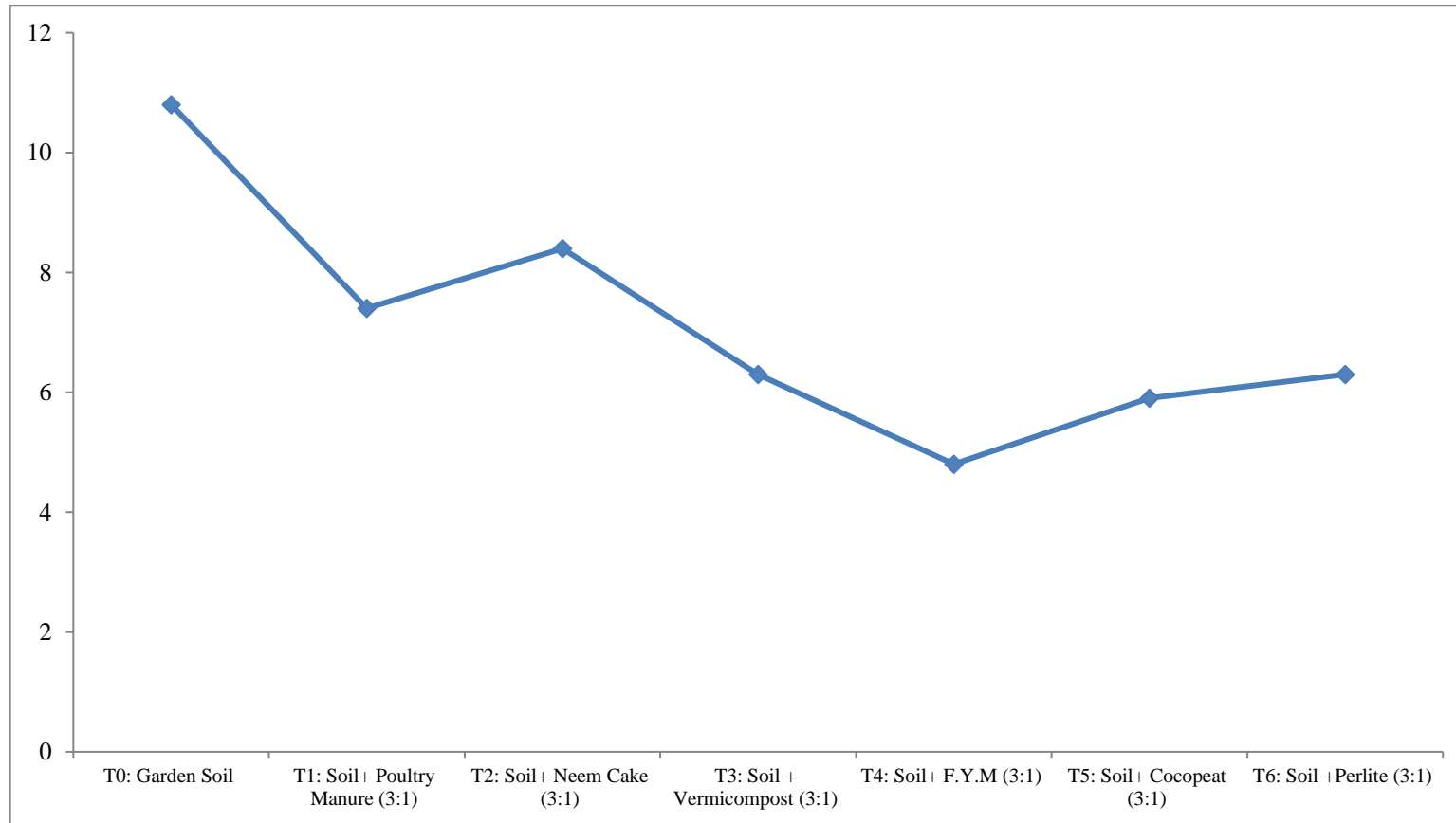
Fig. 3. Effect of treatments on imbibition period of Papaya seeds
