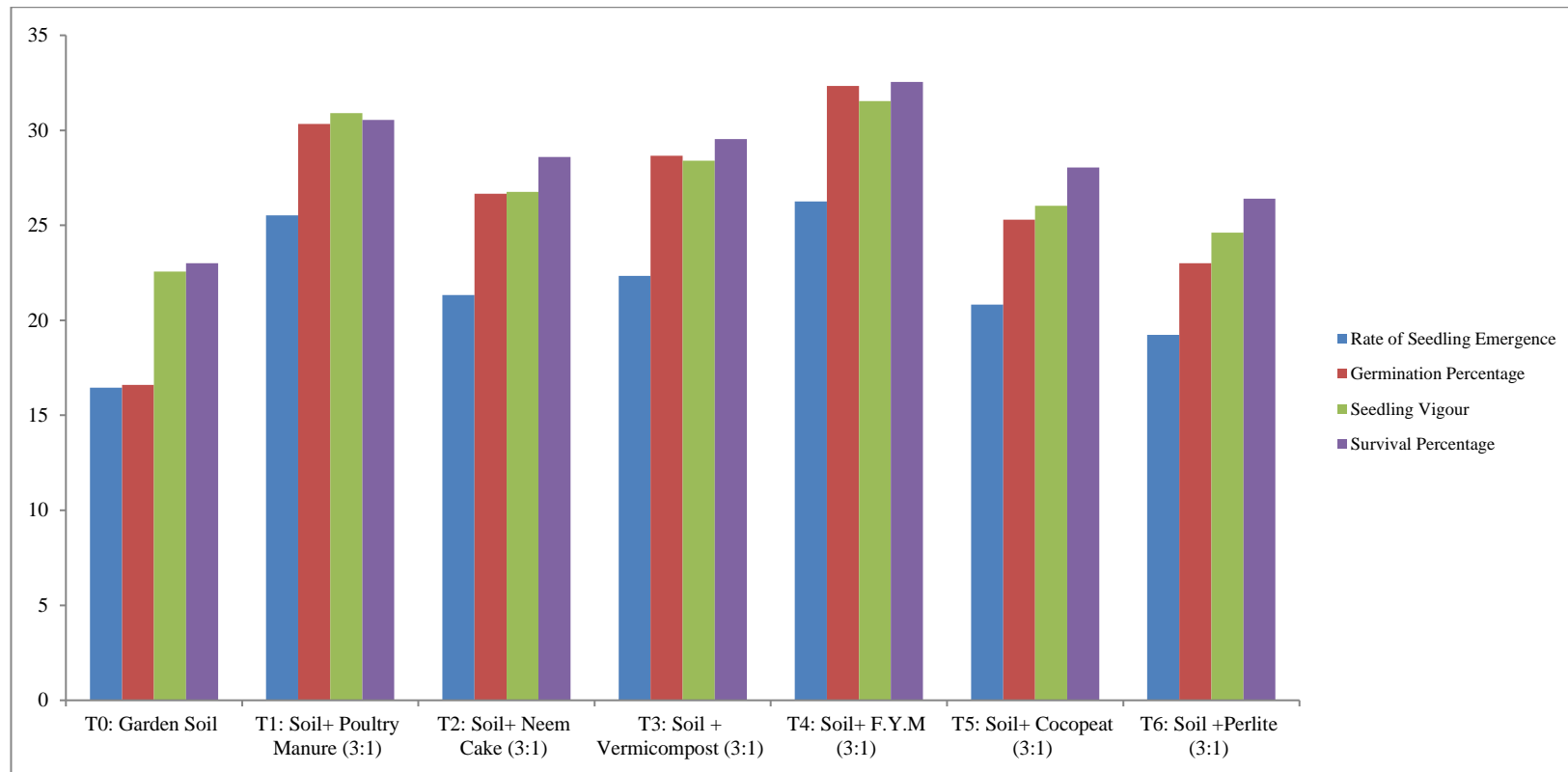
Fig. 1. Effect of treatments on germination parameters of Papaya.
