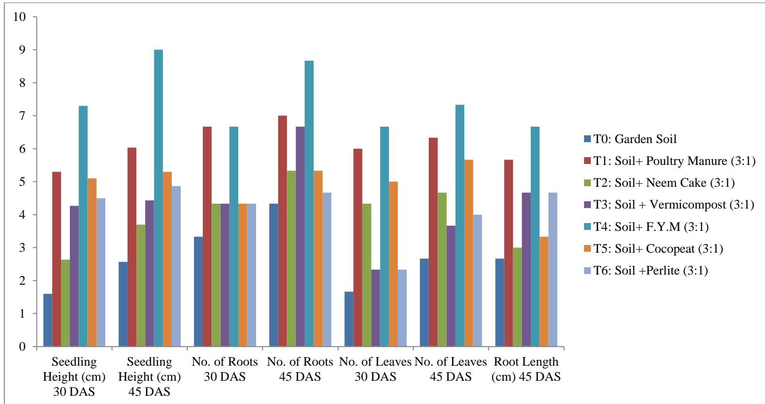
Fig. 2. Effect of treatments on physical parameters of Papaya
